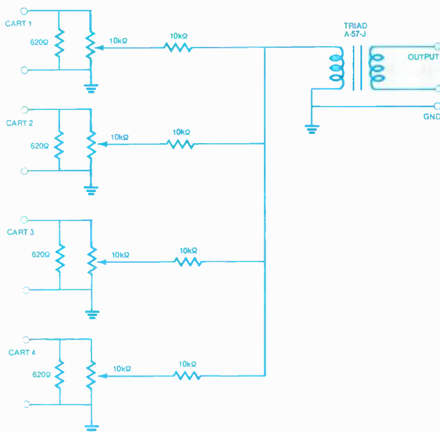
Figure 10. Simple submixer for inputs of a similar nature.
