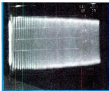
Figure 5(c). Sweep pattern with too little high frequency equalization.
