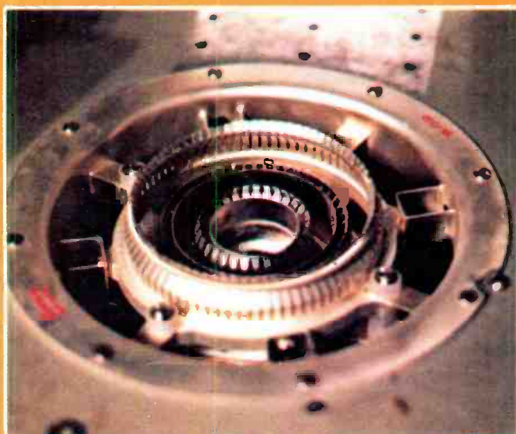
(b) The PA tube socket, just 30 minutes after photo (a) was taken.
