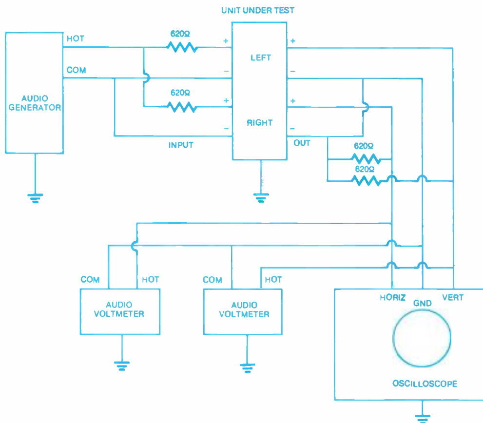
Figure 4. Tape deck alignment test setup.
