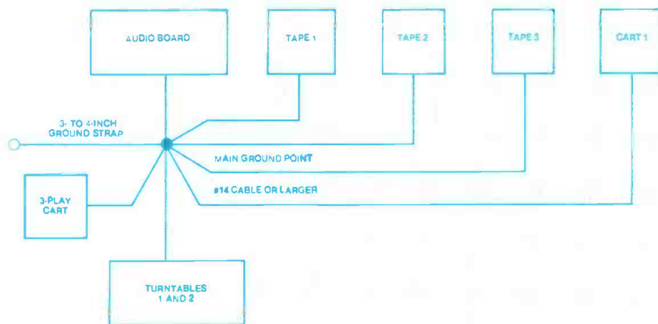
Figure 2. Ground system layout for individual equipment rooms.
