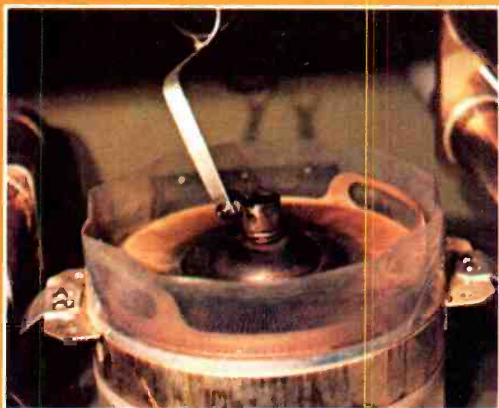
(a) Just before modification. Note discoloration of tube, which had less than 2000 hours on it.
