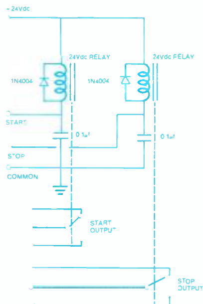
Figure 7. Source control unit.
