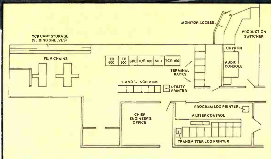
Figure 1. WISH-TV engineering facilities floorplan.
