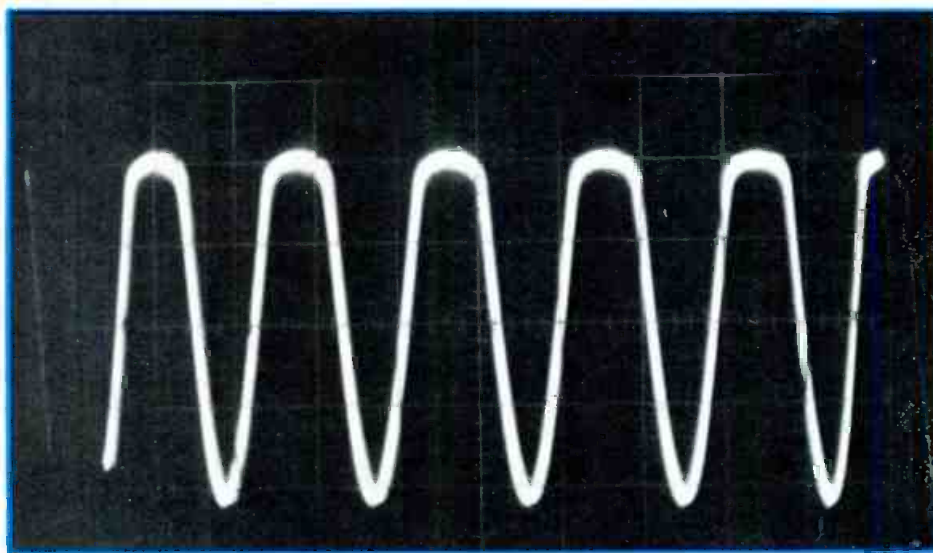
Figure 12. A clipped waveform that can be used to check for proper system phasing.
