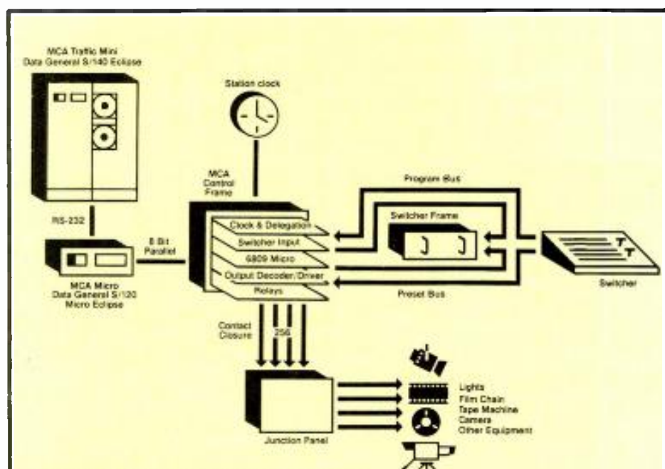
Figure 1. BIAS Master Control Automation.
