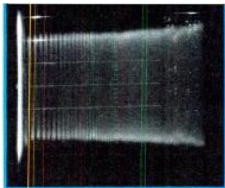
Figure 5(b). Sweep pattern with too much high frequency equalization.
