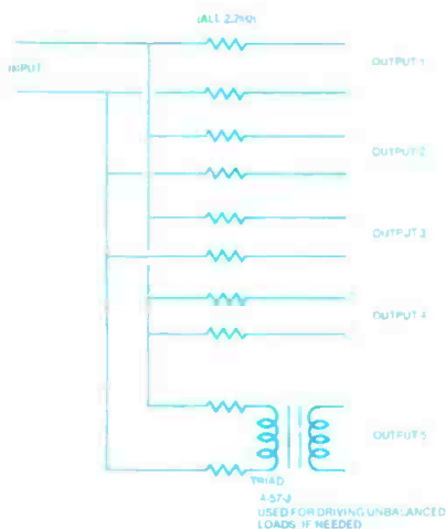
Figure 11. Audio console output distribution board.
