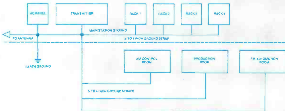
Figure 1. Grounding system layout for radio station with local transmitter.
