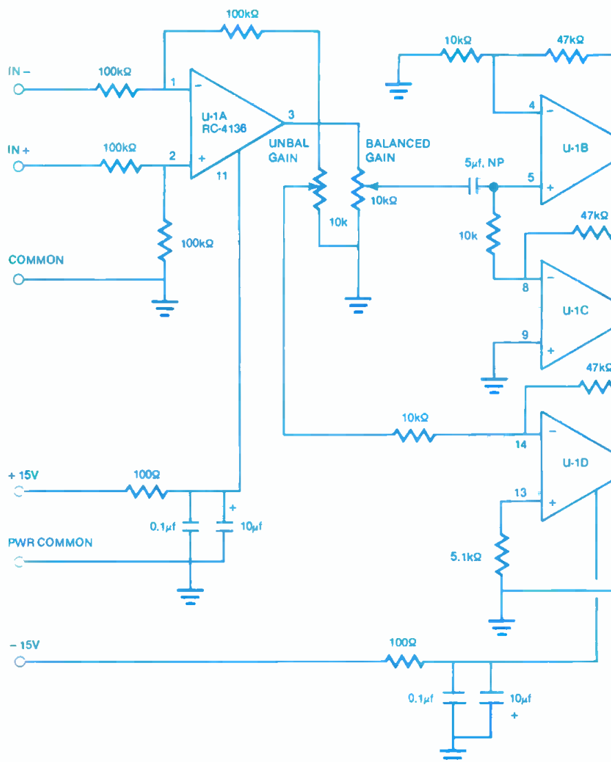
Figure 9. Buffer distribution amplifier.
