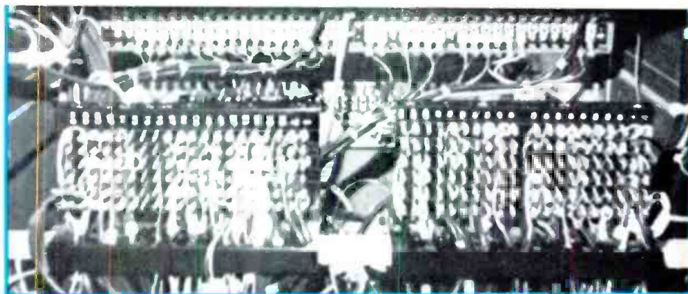
Use of Christmas Tree terminal blocks makes for a neat and easily modified installation.
