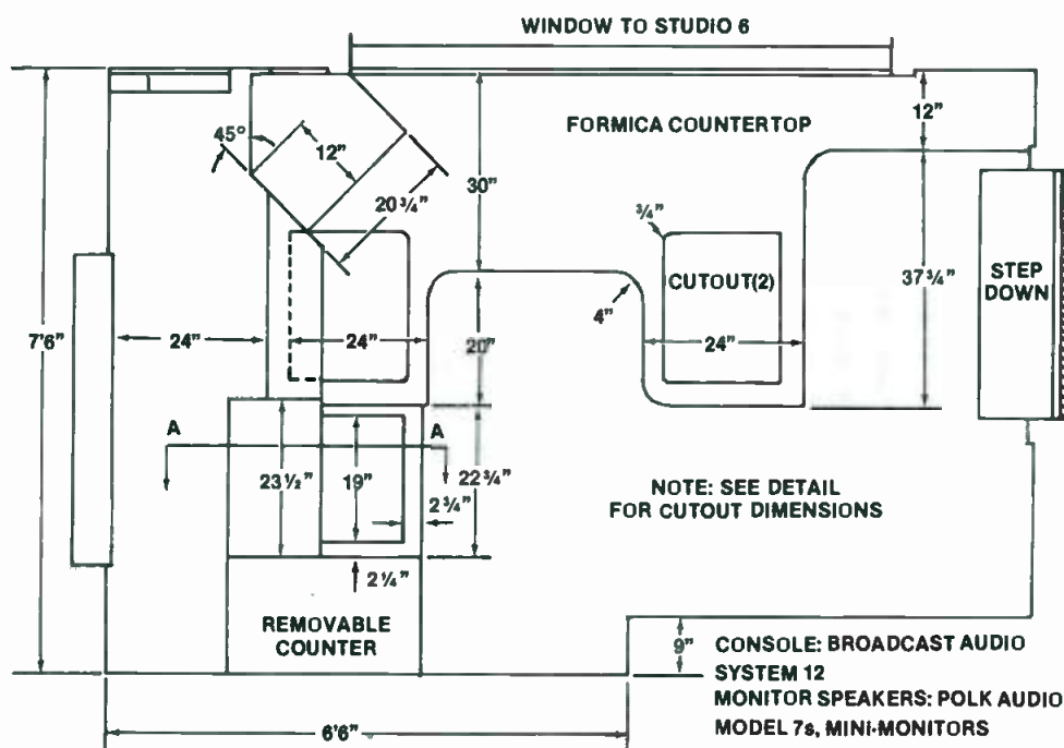
Figure 1. Floor plan for Studio 5.
