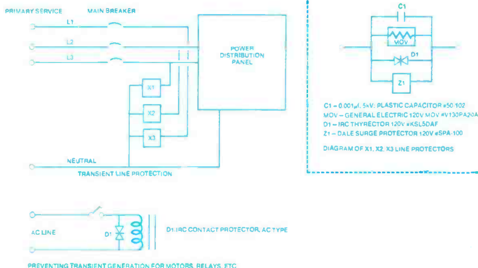
Figure 3. Methods of suppressing transients on the ac power line.
